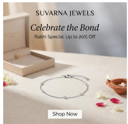
Gemini 3.1 Flash-Lite
