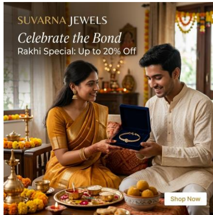
Gemini 3.5 Flash
