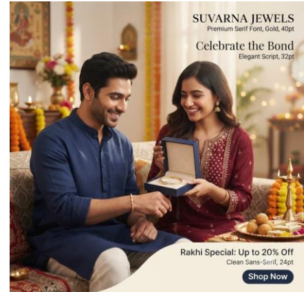
Gemini 3.1 Flash-Lite
